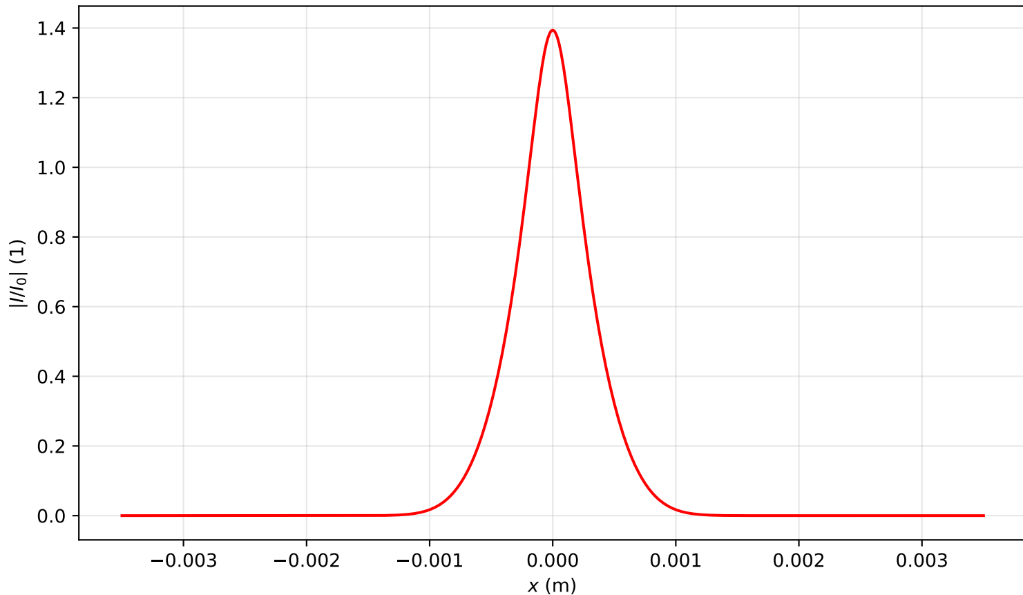
Intensity profile I(x, y = 0, z = 0.239)/I_0 , P_{in}=5.0P_{cr} , artificial time
